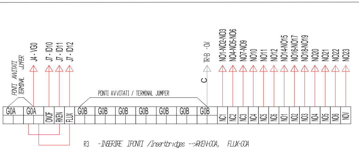
MORSETTIERA UTENTE / USER TERMINAL BOARD (use copper conductor only)
