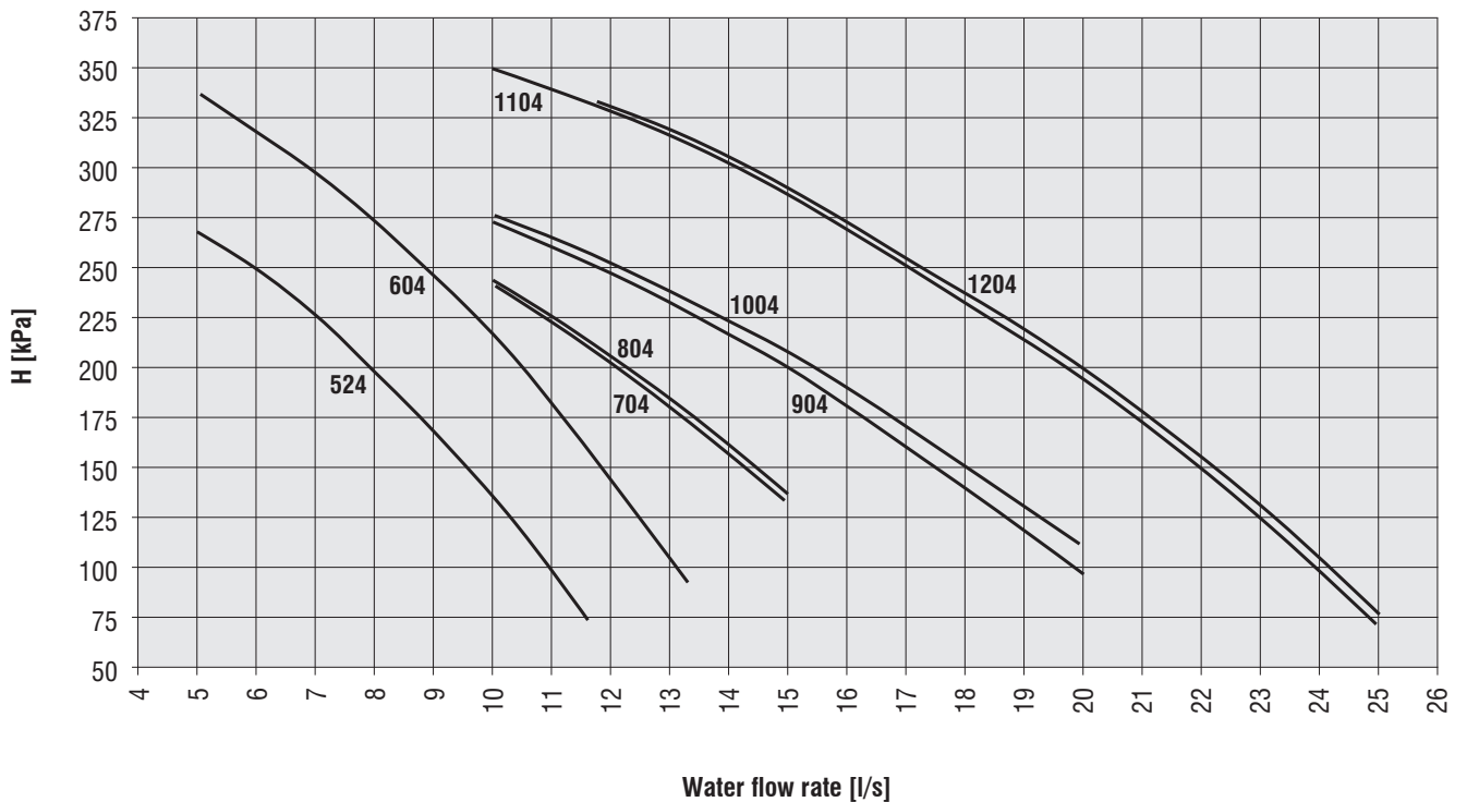
WQL/H 50-190 available static pressure - external heat exchanger (1/2P HP/C)
