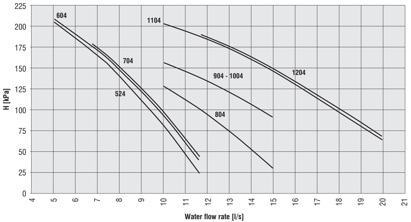
WQL/H/RC 524-1204 available static pressure - internal heat exchanger (1/2P SP/E)
