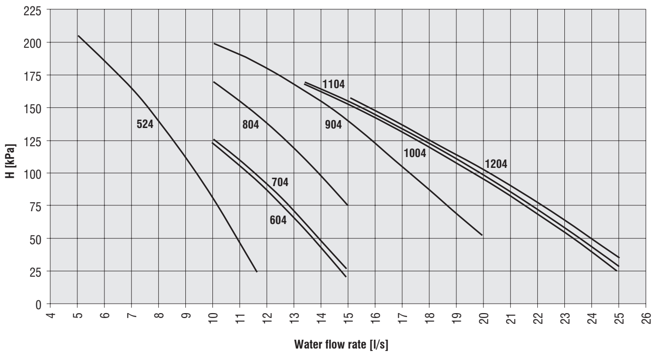
WQL/H 524-1204 available static pressure - external heat exchanger (1/2P SP/C)
